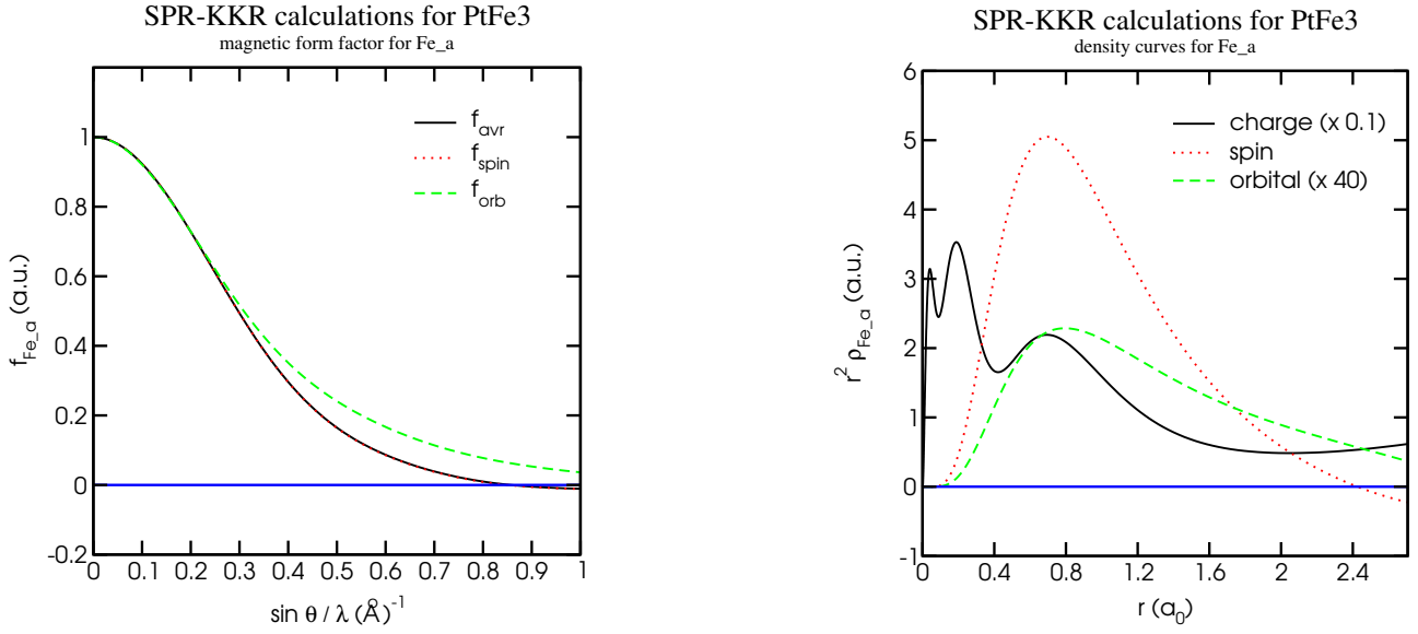
Figure 4.1: Magnetic form factors (left) and density curves (right) for Fe in the ordered compound \text{Fe}_3\text{Pt} .
