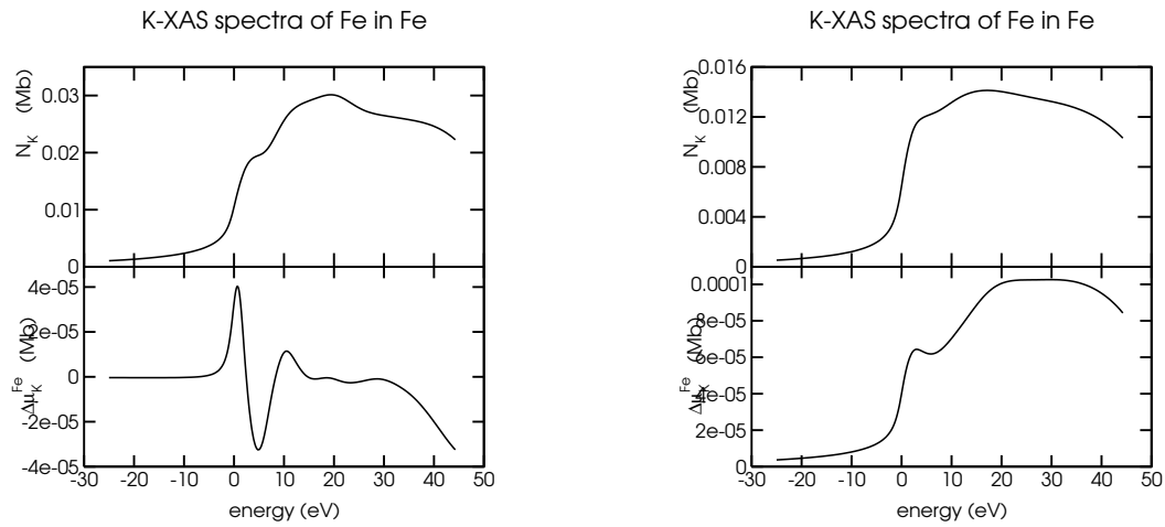
Figure 6.1: X-ray absorption spectrum at the K-edge of Fe in bcc-Fe. Left: results obtained using a Brillouin-zone integration for \tau (program kkrigen ). Right: results obtained by means of a real-space calculation for \tau (program embgen ) with a cluster size of 1.5 a_{\text{Fe}} . Top panel of each figure shows the polarization averaged absorption coefficient \bar{\mu} , the dichroic signal \mu^+ - \mu^- is shown at the bottom. Note: the broadening may lead to artefacts at the high energy end of the spectrum. The cluster calculation is not converged !
