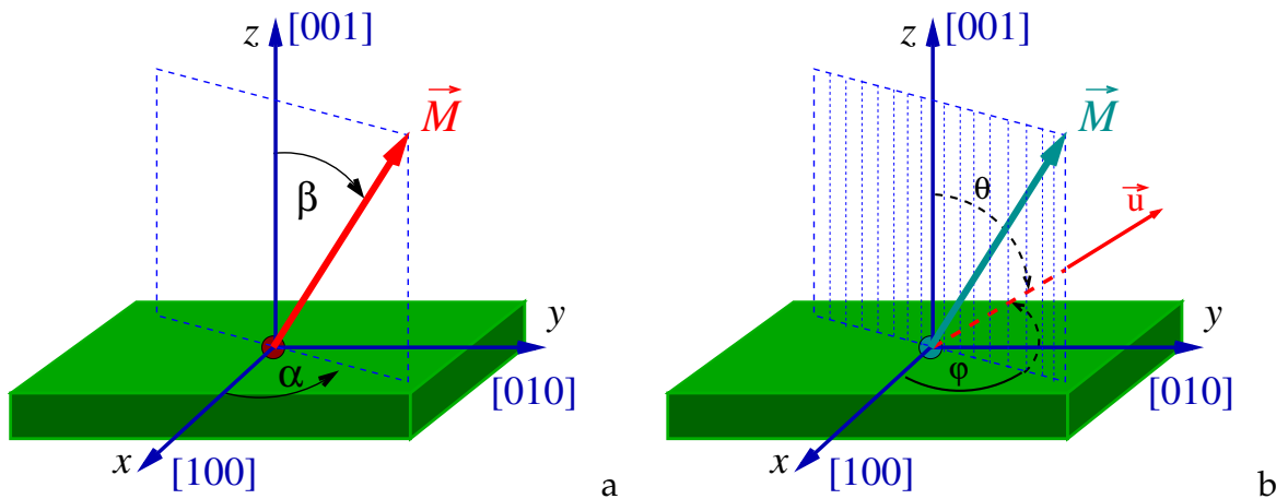
Figure 4.4: Geometry for torque calculations
