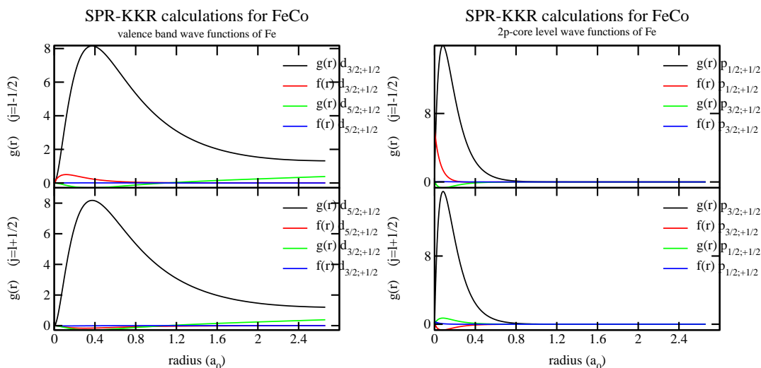
Figure 3.4: The valence band d-electron (left) and 2p-core state (right) wave function for Fe in FeCo. The core wave functions have been created in a second run of kkrgen .
