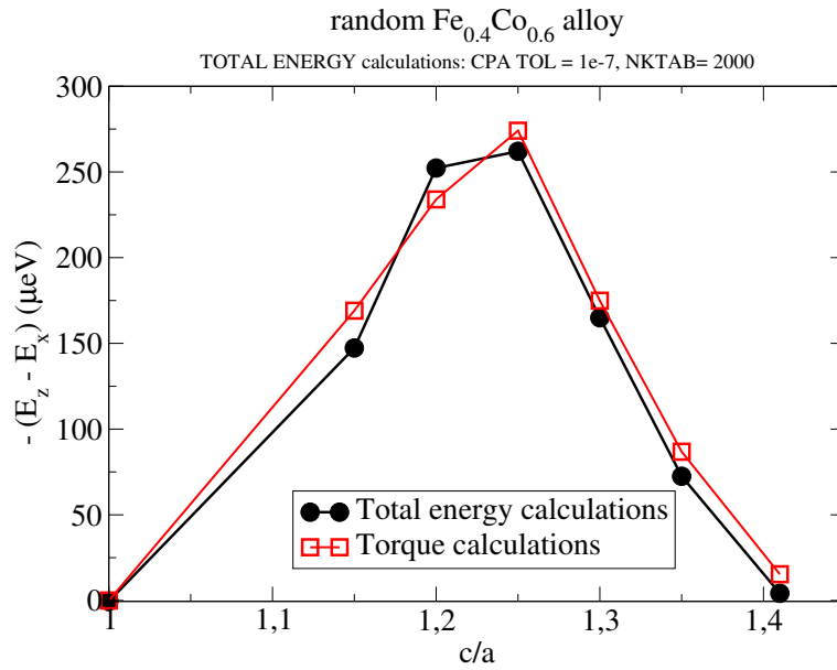
Figure 4.5: MCA for for random bct Fe 0.4 Co 0.6 alloy as a function of the tetragonal strain c/a .
